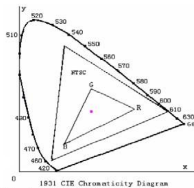
Fig.4. 1931 CIE chromaticity diagram
