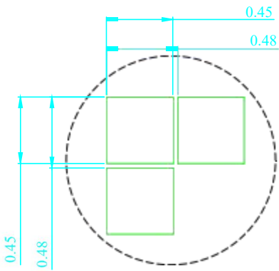
DOTS DETAIL A SCALE 10X
