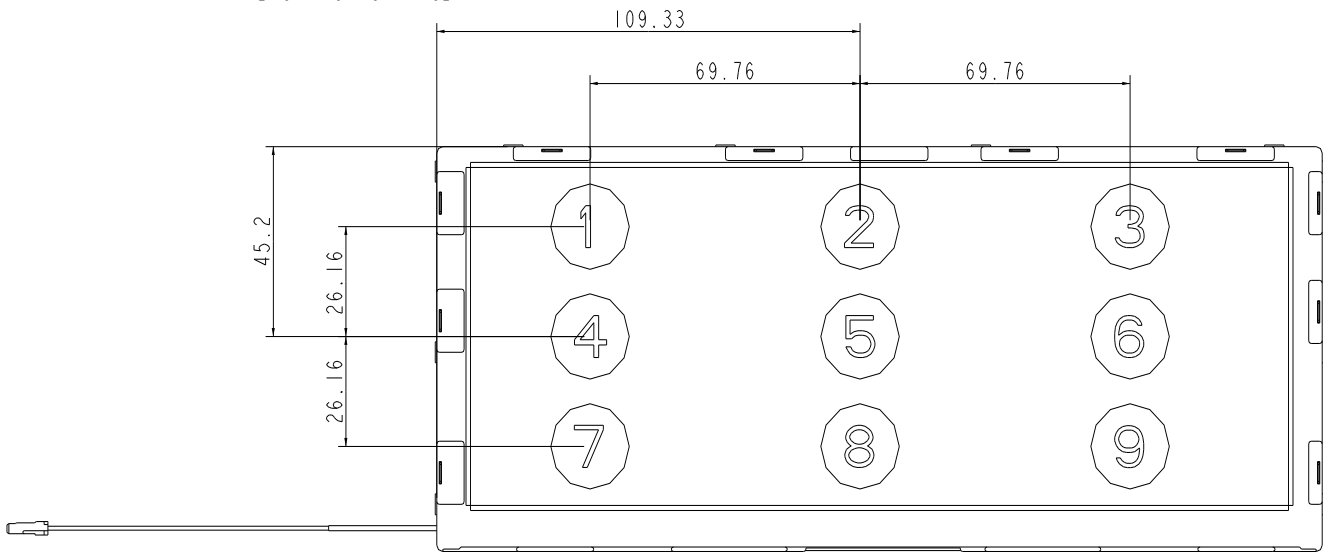
Fig.7-1 Measuring point
